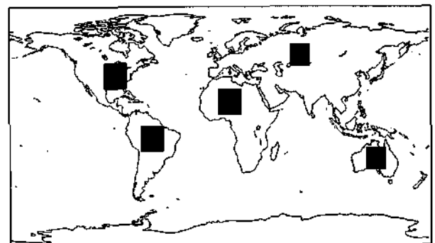
FIG. 8. Location of the five selected continental regions.
