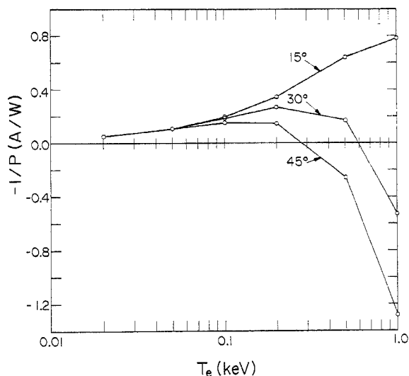
FIG. 5.—Variation of the figure of merit ( I/P ) with the central electron temperature ( T_e(0) ). Different curves show results for different angles of incidence. The angles are measured away from the normal to the magnetic field.
