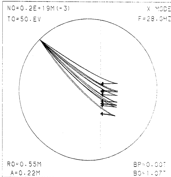
FIG. 1.—Minor cross section projection of ray trajectories. The plasma parameters values are displayed. Each cross on a ray marks a 5% decrease in the power carried by the ray. The vertical dashed line marks the position \omega = \Omega_e(x) . Each ray is launched with a different angle of incidence in a conical pattern with full angular aperture of 20^\circ . In the toroidal direction, the launch angles are in the range 110^\circ \leq \theta \leq 130^\circ (measured with respect to the axial magnetic field).
