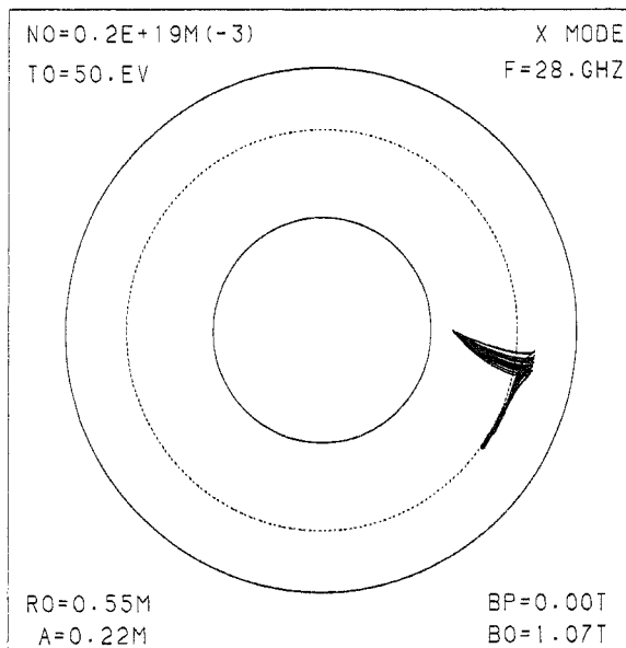
FIG. 2.—Major cross section projection of ray trajectories.
