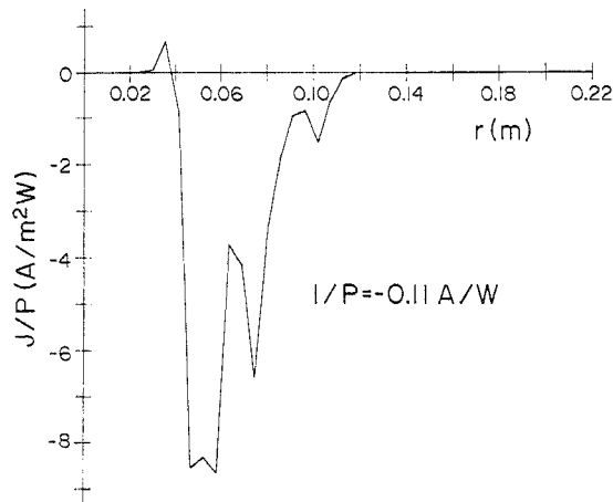
FIG. 4.—Current density profile. The total current is the integral of J(r) over the minor cross section. P is the total incident power.
