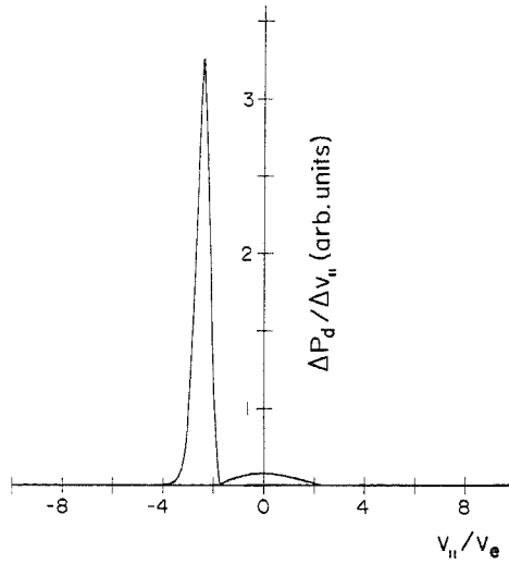
FIG. 3.—Power deposited per unit parallel velocity interval.
