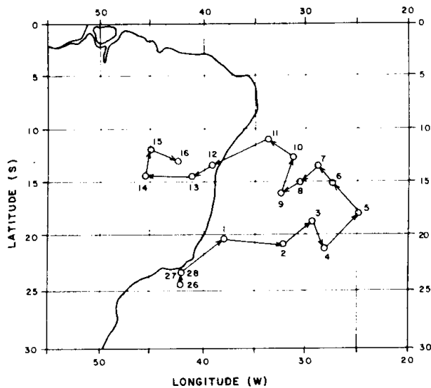
Fig. 5. Path of the 200 mb cyclone 26 February–16 March 1978.
