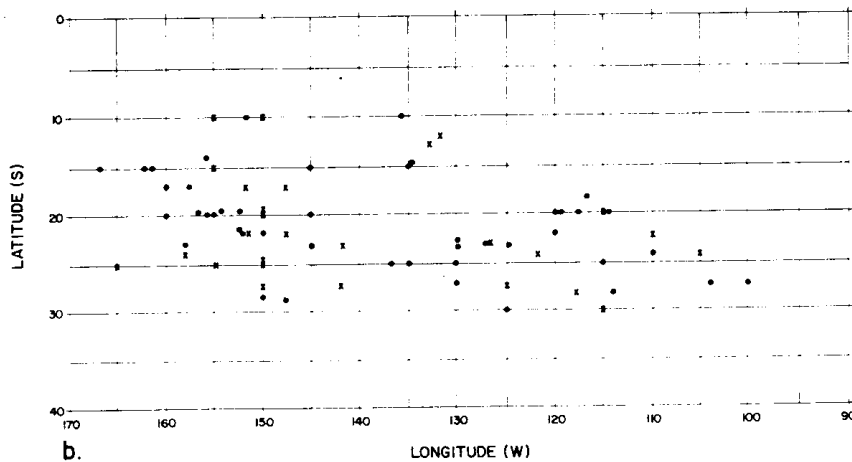
Fig. 1. The positions of subtropical 200 mb closed cyclonic vortices observed in mosaics of polar orbiting satellite data (1975–1979) for the (a) South America–South Atlantic zone and (b) South Pacific region. The position that each vortex had on the first day on which an identifiable circulation existed is indicated by an X. Subsequent positions are indicated by dots.
