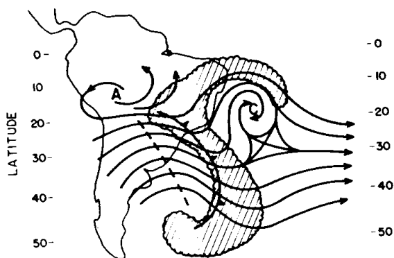
Fig. 7. Schematic illustration of middle and high clouds for the situation in Fig. 6c.
