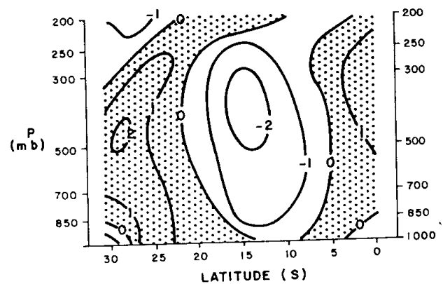
Fig. 3. North–south vertical cross section of temperature departures for 12 March 1978 at 40°W longitude. A longitudinal mean temperature for each level was first computed. Then the departure was determined by taking the NMC grid point temperature and subtracting out the mean. Units are °C.
