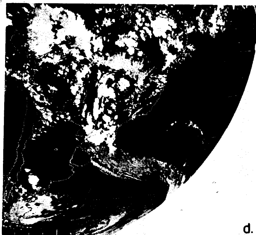
Fig. 8. SMS-2 IR images for 3 March 1980 at (a) 1200 GMT, (b) 1500 GMT, (c) 1800 GMT and (d) 2100 GMT.
