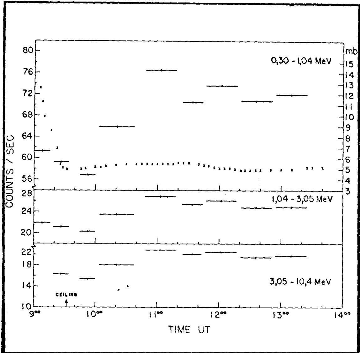
Fig. 2 - Variation of gamma ray counting rate in three different energy bands. The variation of pressure with time is also shown in the figure.
