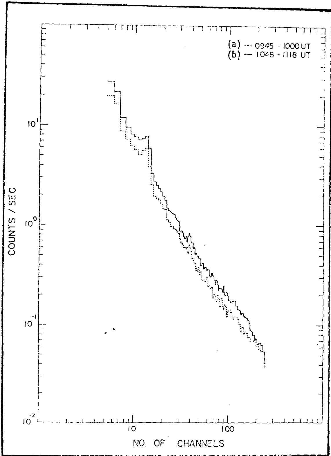
Fig. 3 - Gamma ray spectrum observed immediately after reaching the ceiling (---) and at the maximum counting rate (—).
