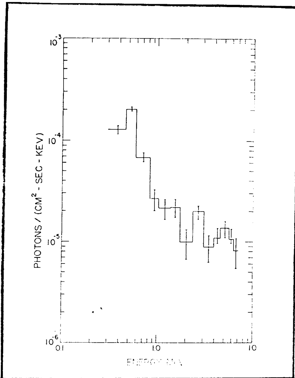
Fig. 5 - Spectrum of the source responsible for the increase in counting rate. The source is suggested to be the supernova remnant in MCG-4-32-23.
