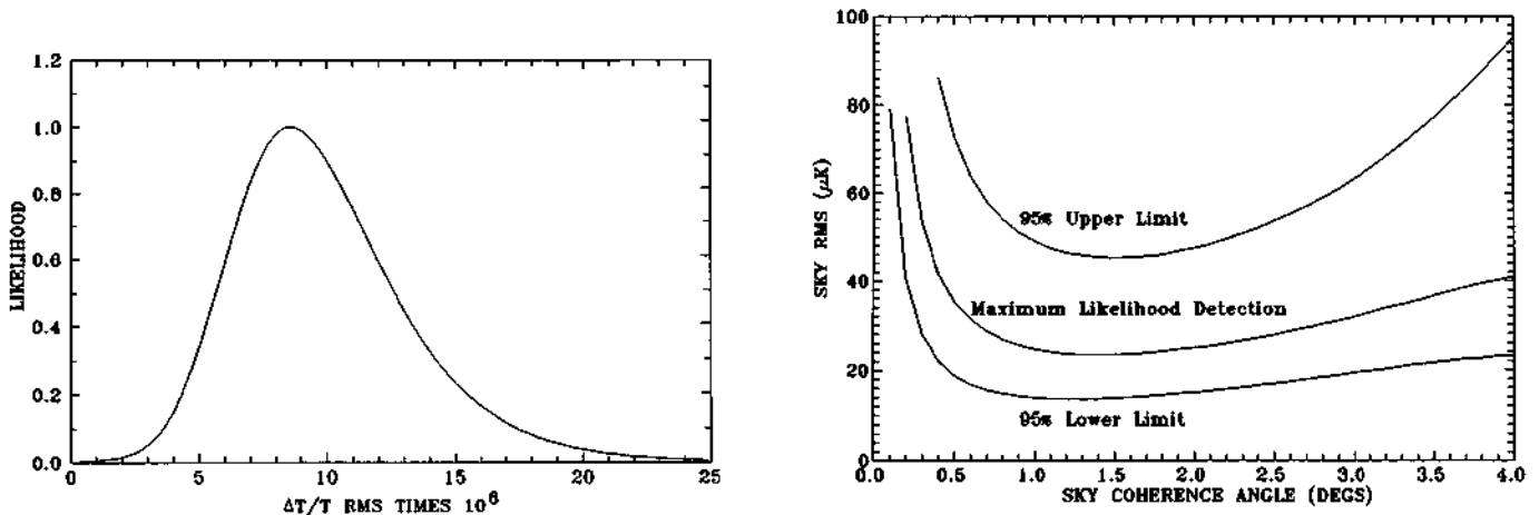
FIG. 3.—95% confidence upper limit, maximum to the likelihood, and 95% confidence lower limit, for an assumed Gaussian sky autocorrelation function
