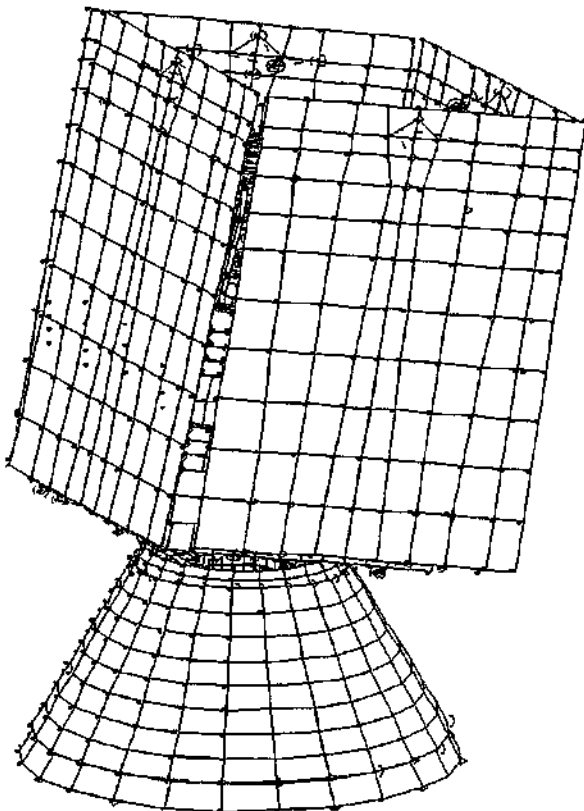
Fig. 14: Mode 2 natural frequency, (38.1 Hz, lateral).
