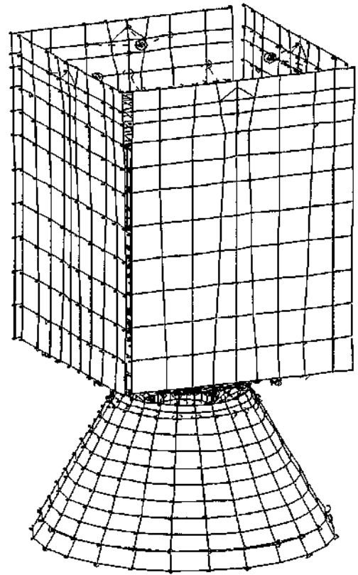
Fig. 15: Mode 3 natural frequency (59.7 Hz, longitudinal).
