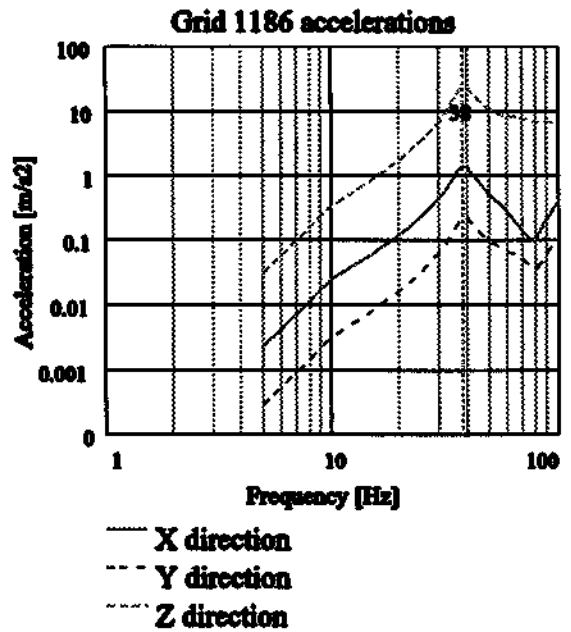
Fig. 21: Grid 1186 accelerations.
