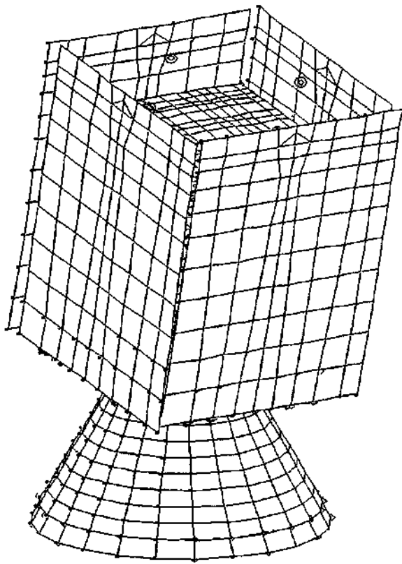
Fig. 13: Mode 1 natural frequency (37 Hz, lateral).
