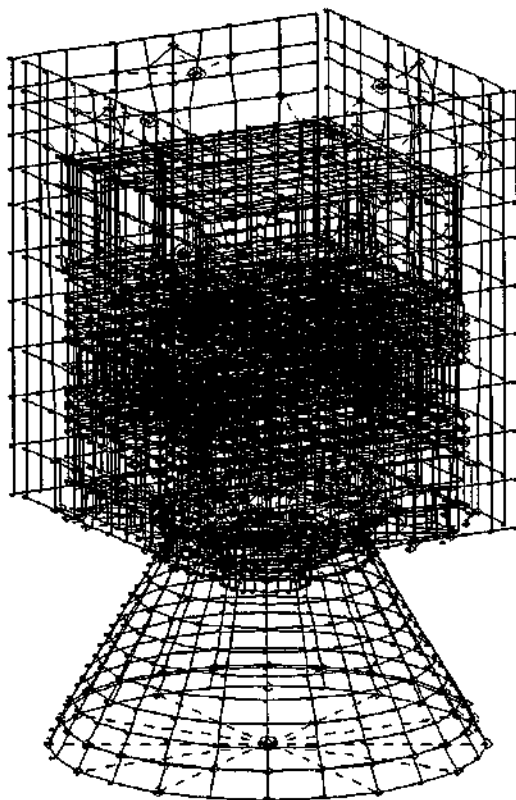
Fig. 8: Full SACI-1 FEM model.
