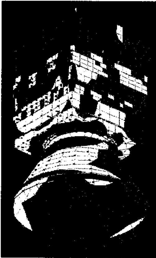
Fig. 10: Case 3. Stresses from 0.01 (green) to 18 (red) MPa.
