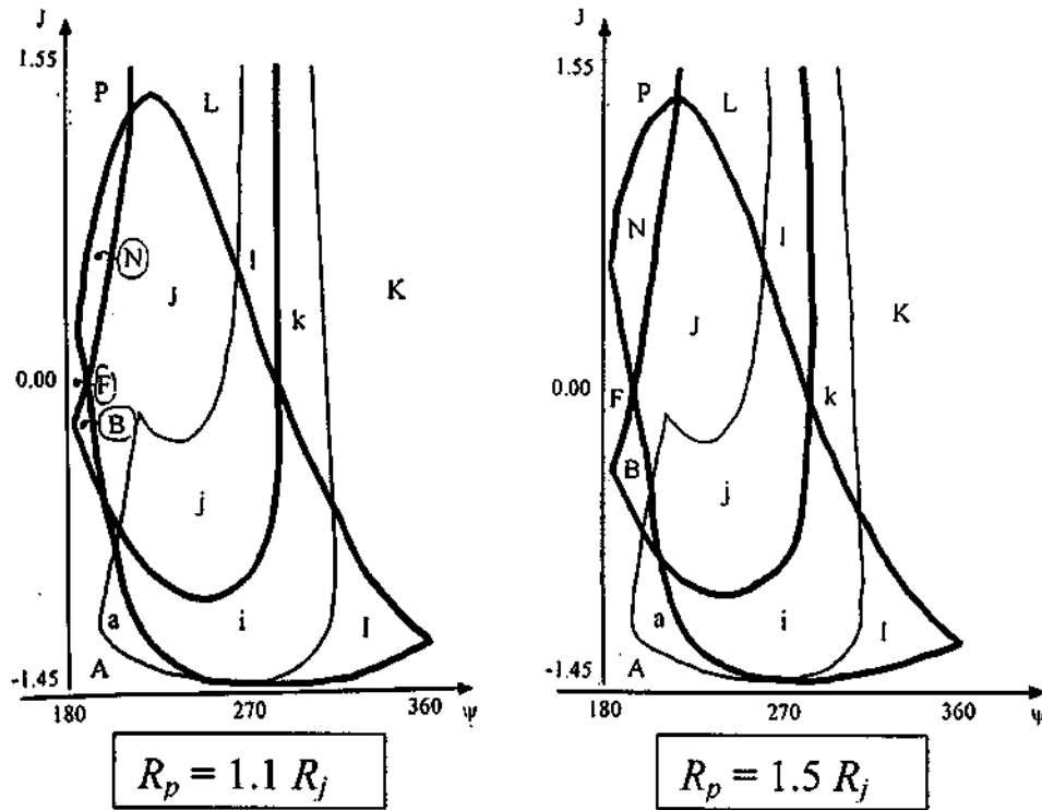
Fig. 2 - Results for R_p = 1.1, 1.5, 2.0, 5.0, 10.0, 50.0 .
