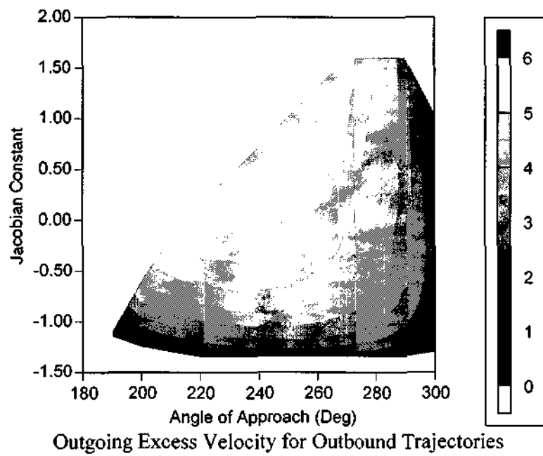
Fig. 5 – Results for the case R_p = 1.1 R_J .
