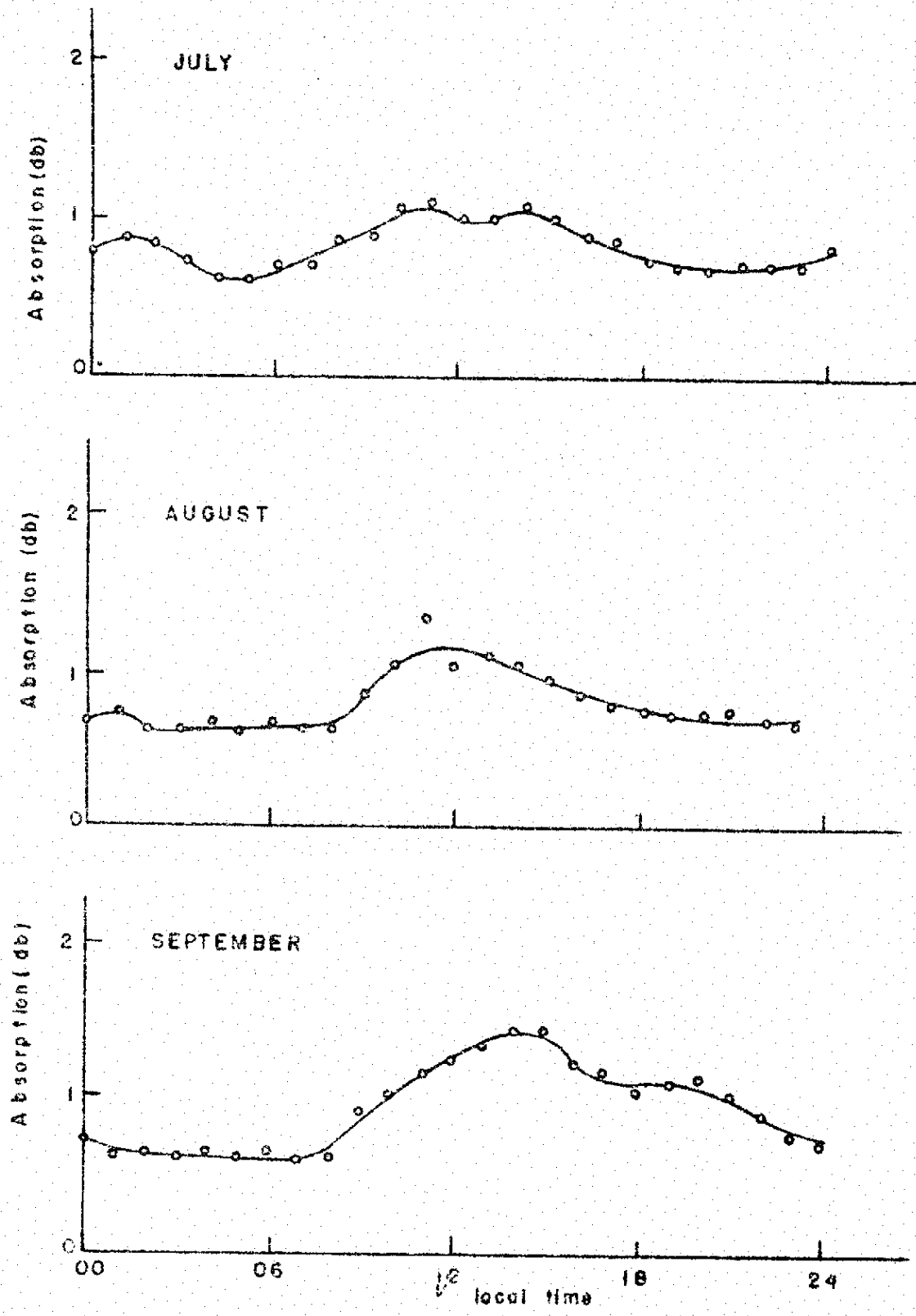
FIG 2 MEDIAN MONTHLY ABSORPTION CURVE (July-September 1966)
