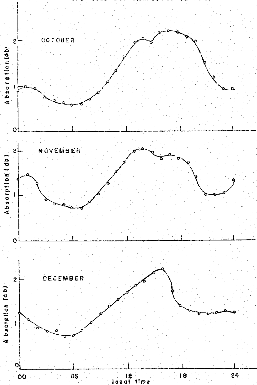
FIG 3 MEDIAN MONTH ABSORPTION CURVES (October-December 1966)
