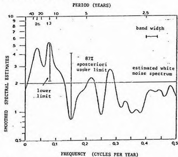
Fig. 1 - Smoothed spectral estimates for Fortaleza annual rainfall time series (1849-1978). The band width of 0.037 was chosen so as to discriminate the frequencies of 1/13 and 1/26.
