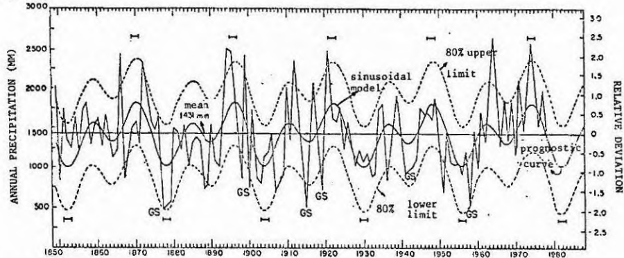
Fig. 2 - Fortaleza annual rainfall from 1849 to 1978 (yearly totals for the hydrological year: November through October). Full continuous line: sinusoidal model with periodicities of 13 and 26 years. Dashed lines: confidence intervals at the 80% level. Dash-dot line: model's prognostic curve for the period 1979-1988. Horizontal bars on the top (bottom) indicate years for which the model would predict precipitation above (below) the average with at least 80% of confidence. Years of extreme droughts ("Grande Seca") are indicated by GS. Relative deviation on the right-hand axis is given by annual precipitation minus the series mean divided by the standard deviation.
