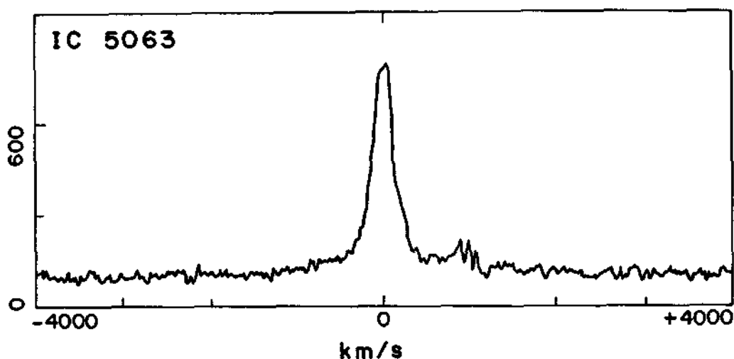
Figure 1. The H \alpha spectrum of IC 5063, after subtracting the [N II] matched by the [O III] \lambda 5007 line.
