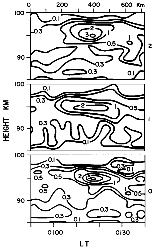
Fig. 5. Na density isopleths for three measuring positions. Contours are marked in units of 10^{10} \text{ m}^{-3} .
