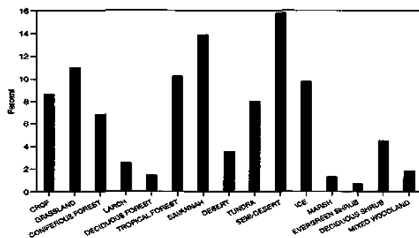
FIG. 1. Fraction of continents covered by the 15 selected land cover types on the T42 GCM grid deduced from the Wilson and Henderson-Sellers (1985) climatology.
