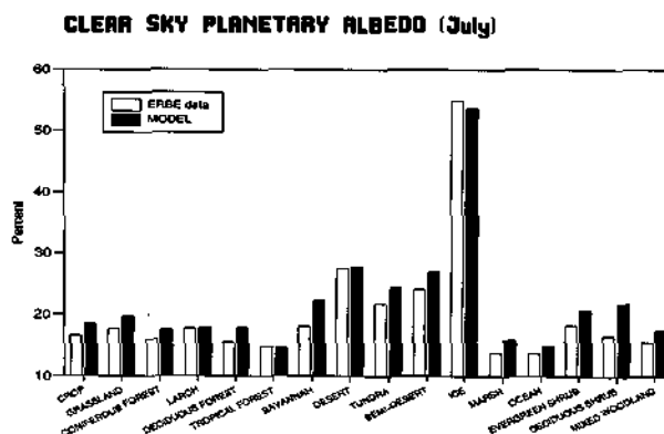
FIG. 3. Comparison of the modeled clear sky planetary albedo with ERBE data in July for each land cover category.
