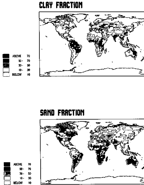
FIG. 2. Maps of the percentage of clay and sand on the T42 GCM grid deduced from the Webb et al. (1991) climatology.
