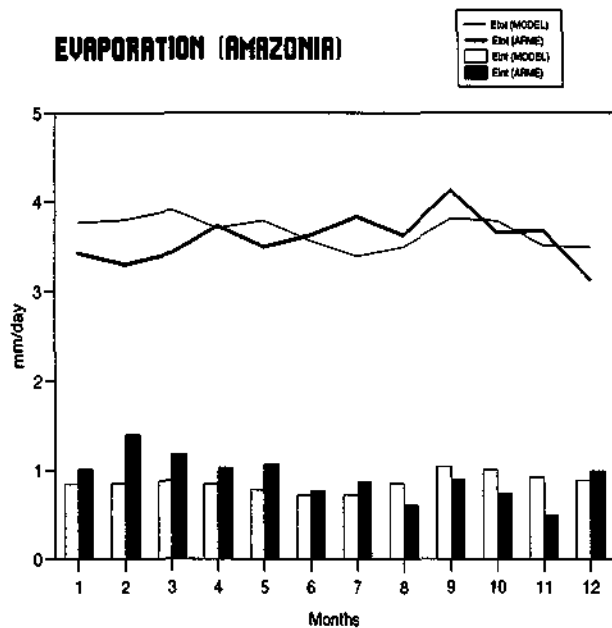
FIG. 11. Mean seasonal cycle of total evaporation and interception loss over the Amazon forest. Simulated cycles are compared with the ARME data from Shuttleworth et al. (1984) and Shuttleworth (1988b).
