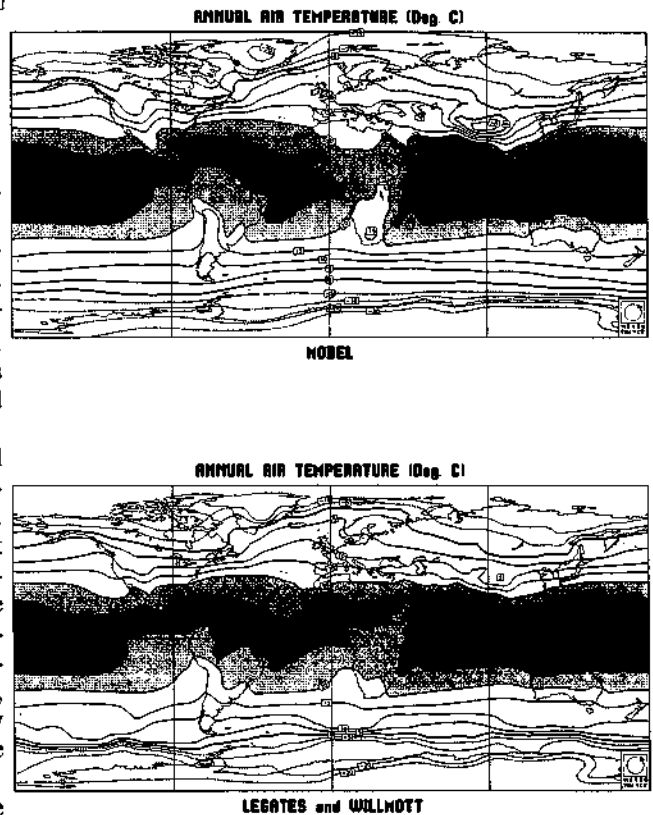
FIG. 5. Mean annual distribution of surface air temperature from the atmospheric model (top) and the observed data of Legates and Willmott (1990b; bottom).
