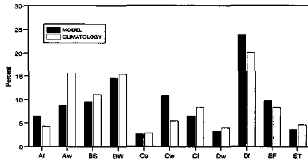
FIG. 6. Fraction of continents covered by the different Köppen climate zones for observations (Legates and Willmott 1990a,b) and the model simulation.
