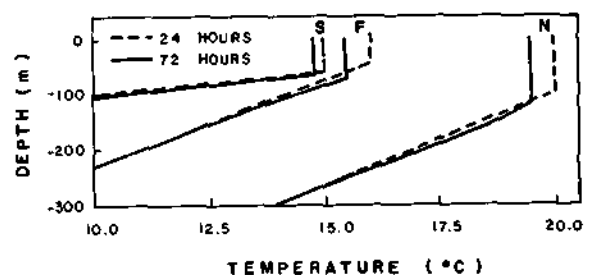
Figure 10. Temperature profiles in the regions south (S) and north (N) of the front and also the temperature profiles in the frontal region (F), when the storm starts (dashed line) and when it ends (solid line).
