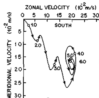
Figure 16. Velocity hodograph in region S. The numbers indicate local inertial periods, and the arrows indicate the direction (the inertial period for 40^\circ\text{S} is 18.6 hours).
