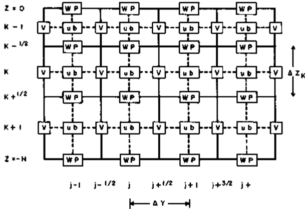
Figure 2. Distribution of the variables on the grid in the y-z plane.
