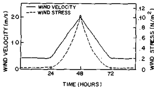
Figure 5. Time variation of the wind velocity, u_a (solid line), and wind stress, |\tau| (dashed line).
