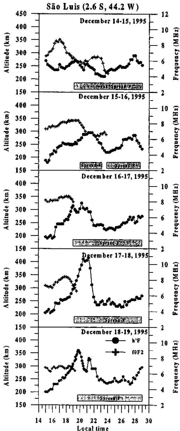
Fig. 6A–E. Local time variations of the ionospheric parameters h'F and foF2 obtained at São Luis ( 2.6^{\circ}S , 44.2^{\circ}W ) for all nights during this campaign: A December 14–15, 1995; B December 15–16, 1995; C December 16–17, 1995; D December 17–18, 1995 and E December 18–19, 1995
