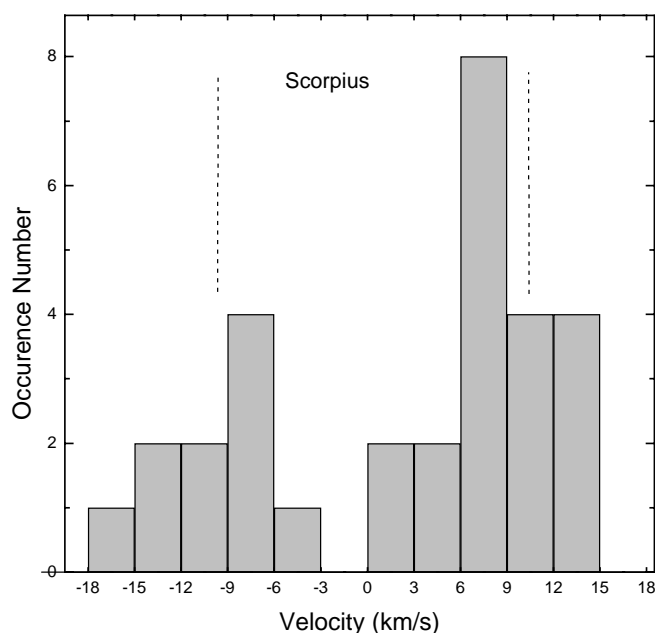
FIG. 4.—Histogram of the radial velocity distribution observed toward Scorpius. Two peaks with radial velocities around -7.5 and 7.5 \text{ km s}^{-1} are seen. The dotted lines show a model of an expanding ring with an expansion velocity of 10 \text{ km s}^{-1} (de Geus 1988).
