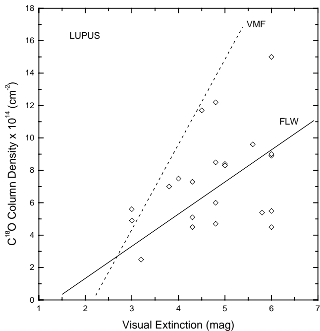
FIG. 1.— \text{C}^{18}\text{O} column density vs. visual extinction for the positions observed toward the Lupus complex. The solid and dashed lines are column density vs. extinction obtained by Frerking et al. (1982, “FLW”) and VMF in Musca, respectively.
