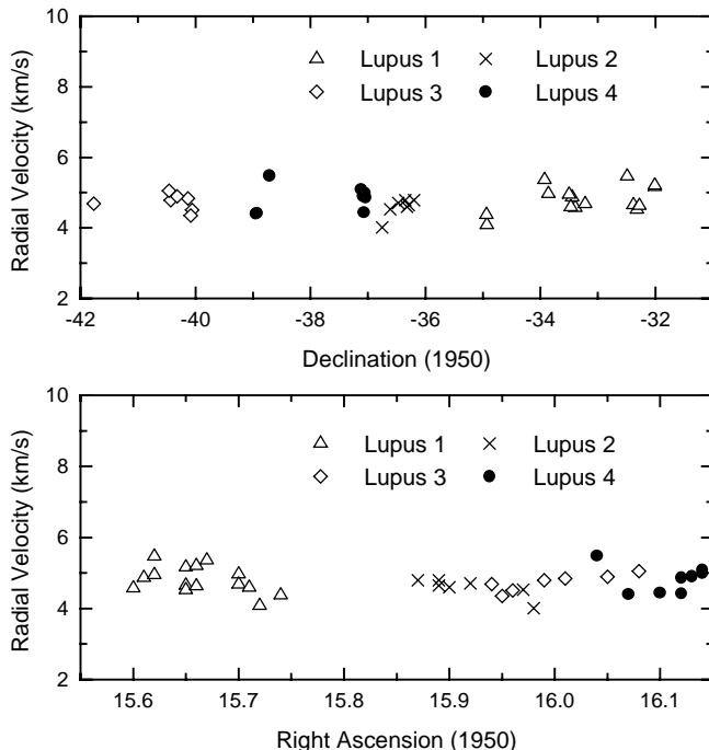
FIG. 2.—Radial velocity vs. right ascension and declination for the condensations observed toward the four Lupus filaments.
