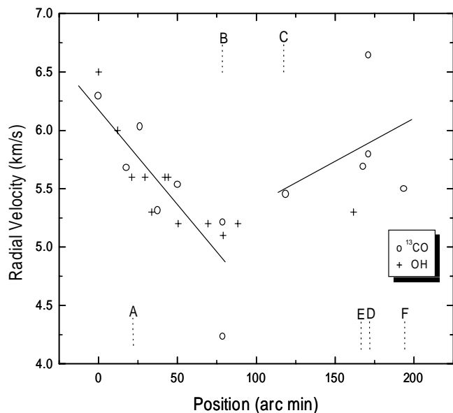
FIG. 5.—Radial velocity vs. position for the condensations observed toward Corona Australis, showing ^{13}\text{CO} radial velocities observed in this survey ( open circles ), OH radial velocities observed by Cappa de Nicolau & Pöppel (1991; crosses ), and the positions of the structures A to F defined by AV as regions with visual extinction higher than 3 mag ( vertical dashed lines ).
