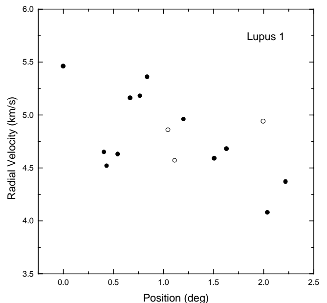
FIG. 3.—Radial velocity vs. position for the condensations observed toward Lupus 1, located along the main filament (filled circles) in an extended structure southwest of this filament (open circles).
