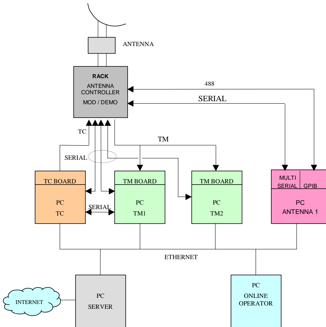
Figure 1: SACI Ground System Architecture
