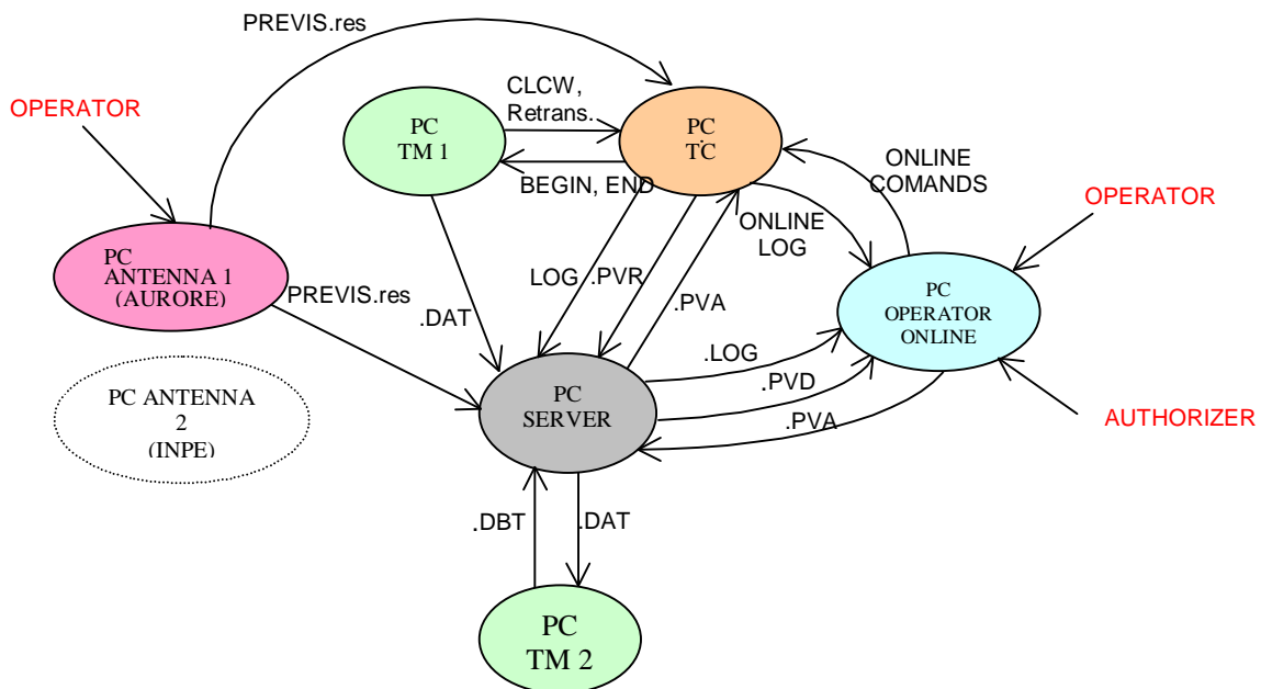
Figure 2: Automatic Ground Station Operation Diagram
