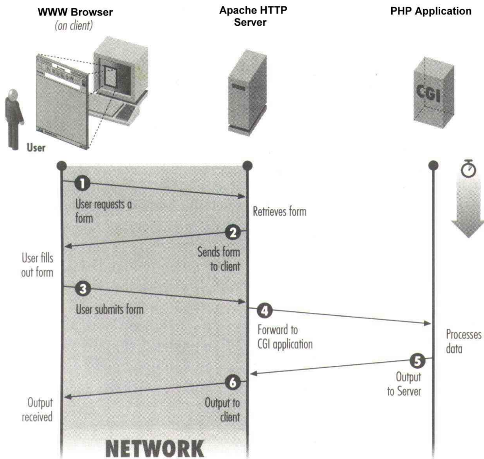
Figure 3 – CGI Process for Preparing the SACI Fight Plan via WWW
