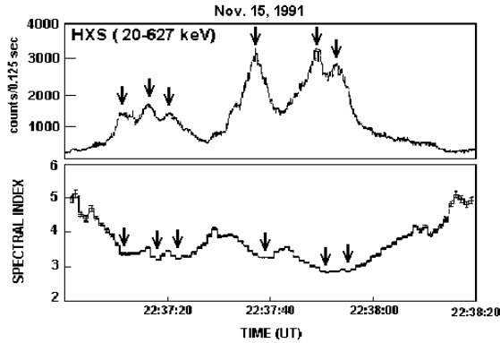
Fig. 4. Top: time profile of hard X-ray flare observed in 1991 November 15. Bottom: time evolution of the spectral index. Each individual peak shows a spectral index evolution as “soft-hard-soft”.
