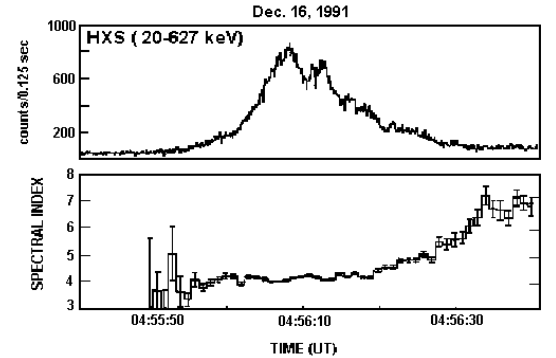
Fig. 5. Top: time profile of hard X-ray flare observed in 1991 December 16. Bottom: time evolution of the spectral index. The global behavior of the spectral index shows an evolution as “hard-hard-soft”.
