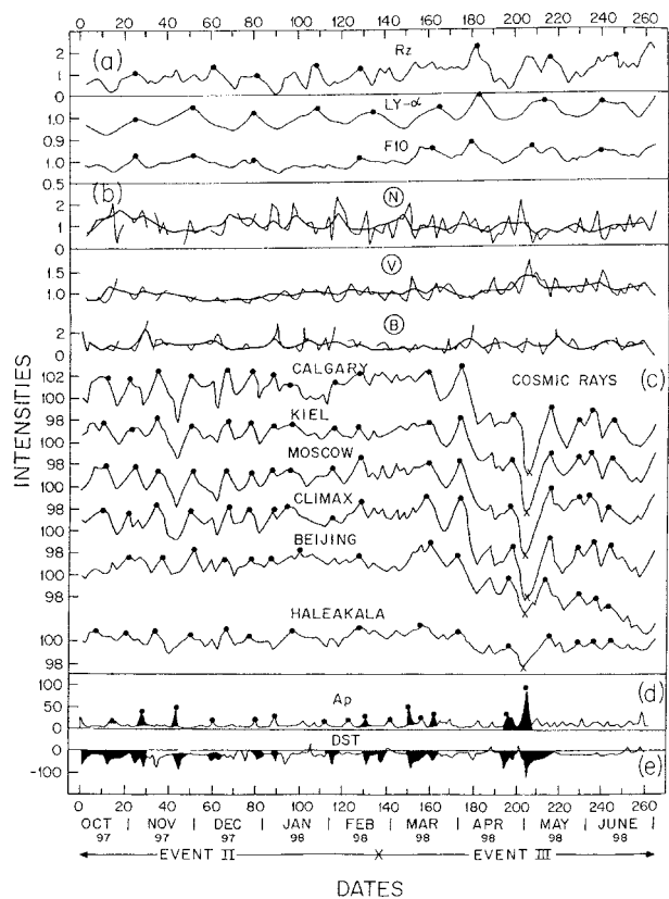
Figure 6. Plots of the percentage deviations of daily values (thin lines) and their 12-month moving averages (superposed thick lines) for (a) solar indices Sunspots (Rz), Lyman alpha, and 2800 MHz flux (F10), (b) Interplanetary parameters N (number density), V (wind speed), B (magnetic field) (c) Cosmic ray neutron monitor intensities at Calgary, Kiel, Moscow, Climax, Beijing, and Haleakala, (d, e) Geomagnetic indices Ap and Dst, for the period 11 October 1997–1 July 1998, events II and III, 264 days.
