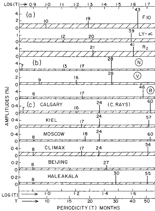
Figure 5. Spectra (amplitudes versus periodicities T in months) for the series of percentage deviations of monthly values for (a) solar indices Sunspots (Rz), Lyman alpha, and 2800 MHz flux (F10), (b) Interplanetary parameters N (number density), V (wind speed), B (magnetic field) (c) Cosmic ray neutron monitor intensities at Calgary, Kiel, Moscow, Climax, Beijing, and Haleakala. The hatched portion indicates the 2\sigma limit and amplitudes protruding above the hatched area are significant at a better than 95% confidence level. Note that the abscissa scale is log (T).
