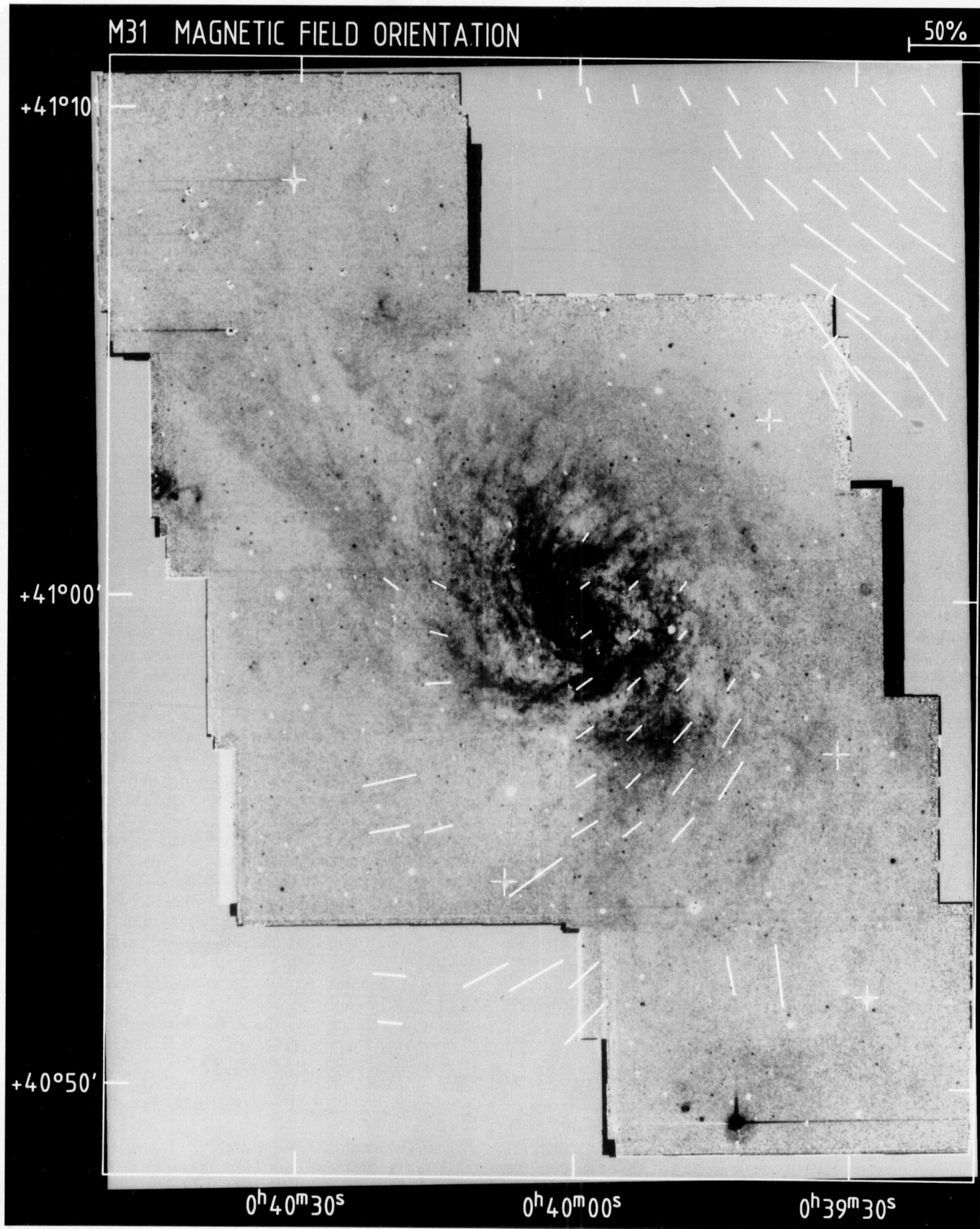
Fig. 11. Orientation of the magnetic field ( \chi_B ) in the central region of M31 overlaid onto the H \alpha photograph of Ciardullo et al. (1988). The lengths of the vectors indicate the degree of linear polarization at \lambda 6.3 cm
