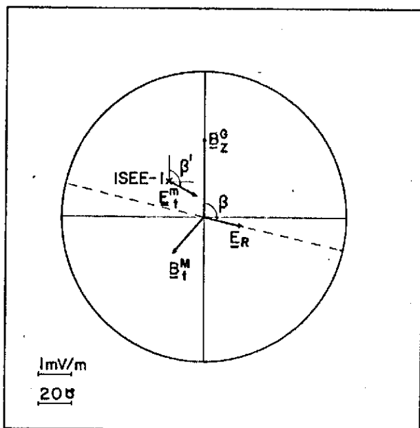
Fig. 1 A view from the sun of the average B^G and B_t^M -fields measured by the ISEE-1 satellite, whose position during the magnetopause crossings is indicated by the x-mark. The dashed line is the computed reconnection line. See text about the angles \beta and \beta' and about the fields E_t^M and E_R .
