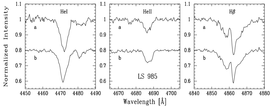
Figure 3. He I 4471 Å, He II 4686 Å and H \beta in the spectrum of the double-lined O-type binary LS 985 at two different observing dates: (a) JD 244 9369.698, and (b) JD 244 9382.601.
